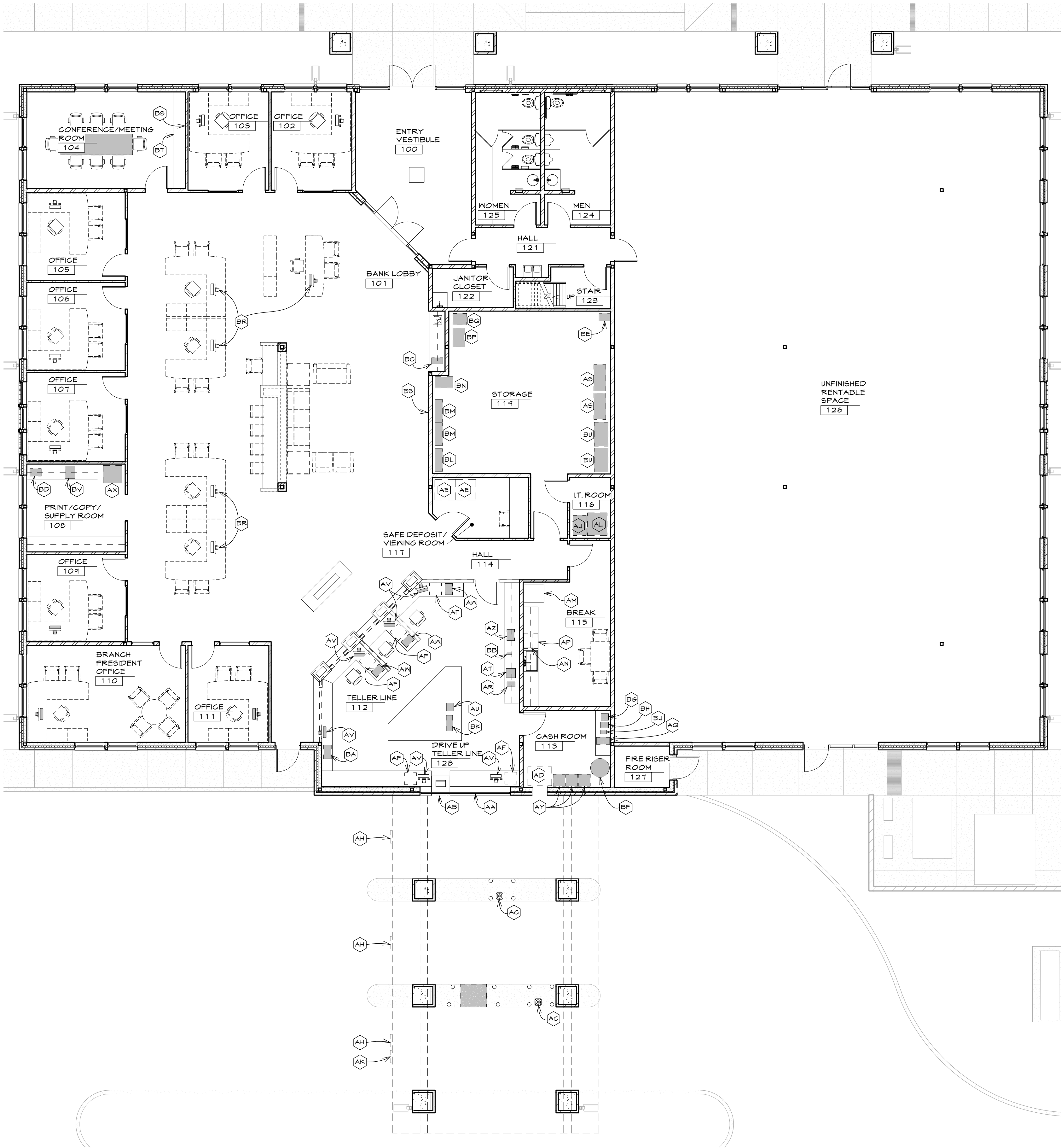
FURNITURE LAYOUT AND EQUIPMENT FLOOR PLAN
