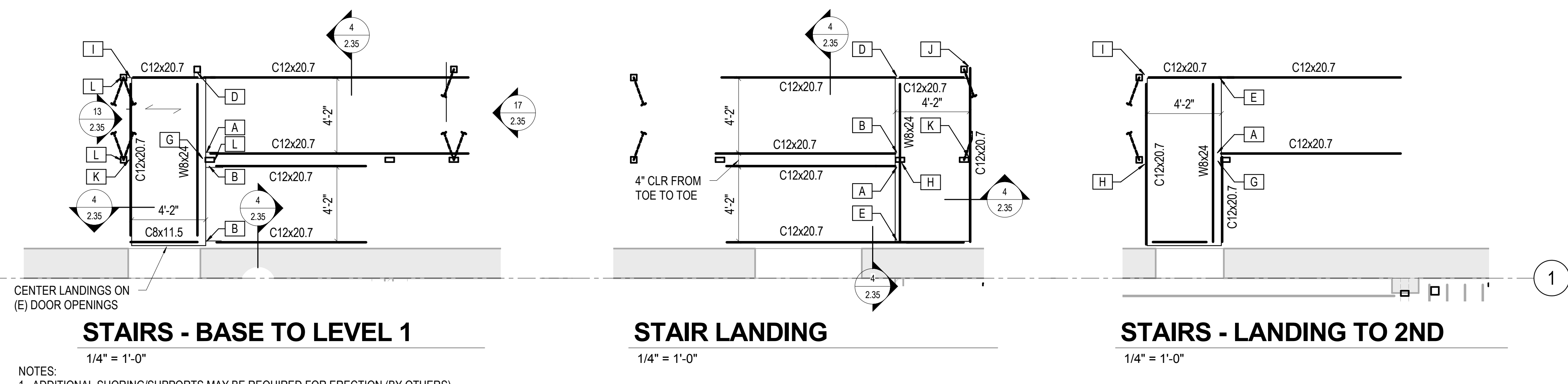
STAIRS - BASE TO LEVEL 1 1/4" = 1'-0" STAIR LANDING 1/4" = 1'-0" STAIRS - LANDING TO 2ND 1/4" = 1'-0"
