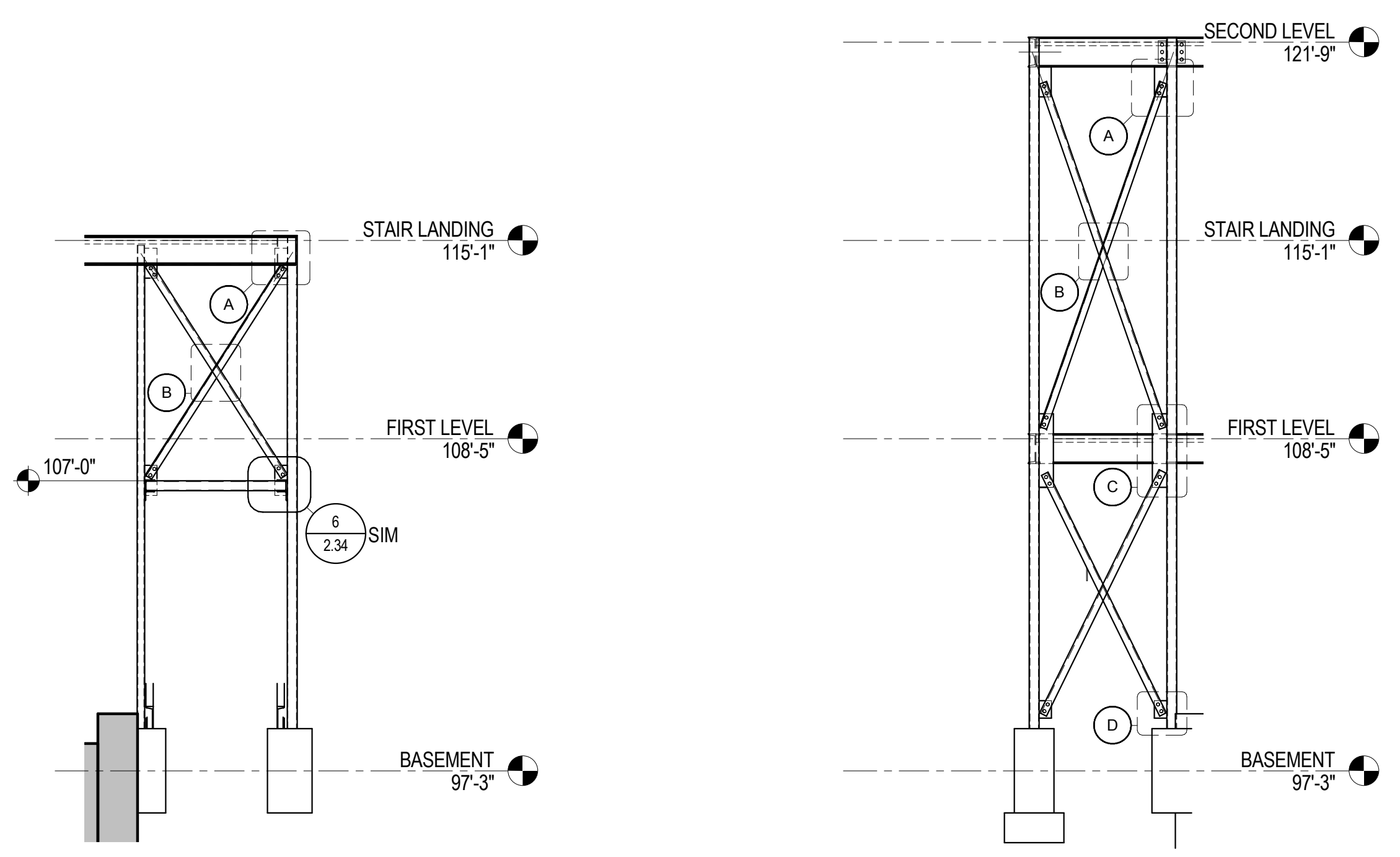
17 STAIR - SOUTH FRAME 1/4" = 1'-0"
