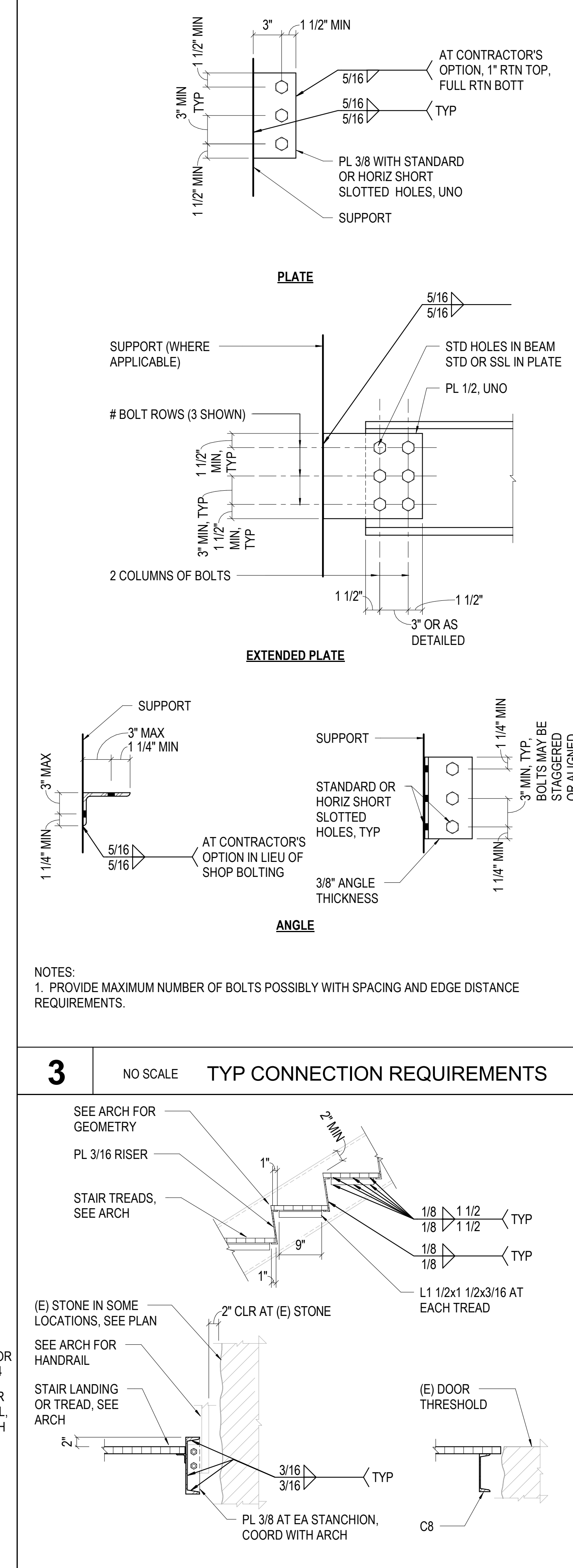
4 NO SCALE STAIR TREADS & LANDING DETAILS
