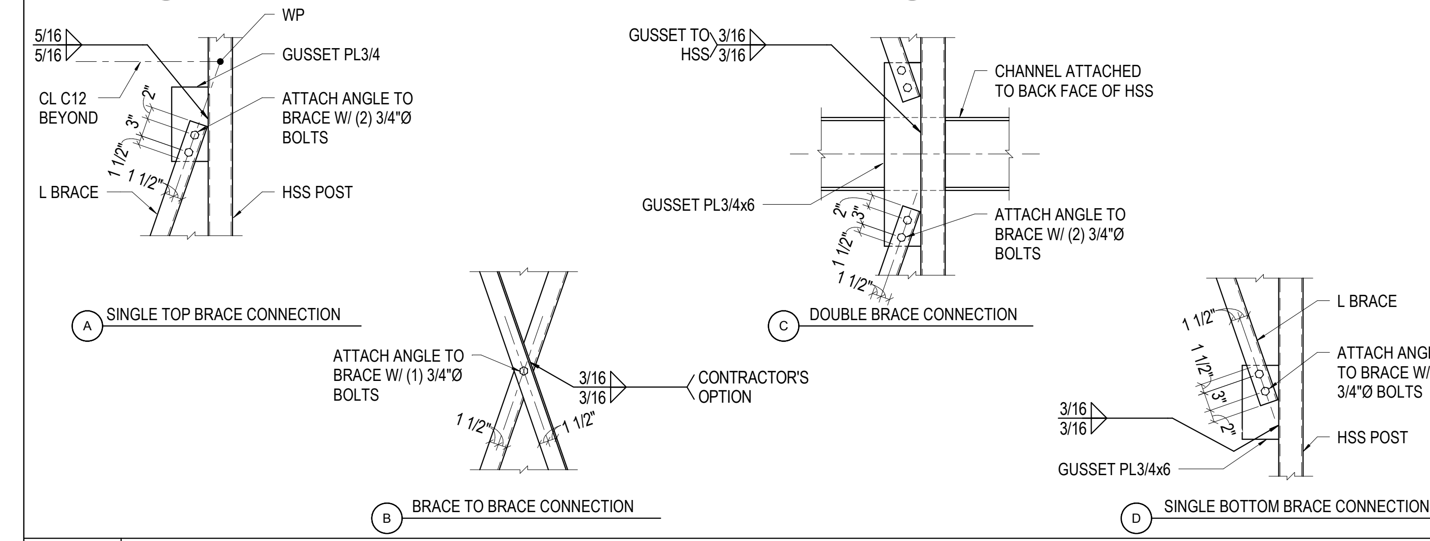
18 NO SCALE STAIR FRAME BRACE CONNECTIONS
