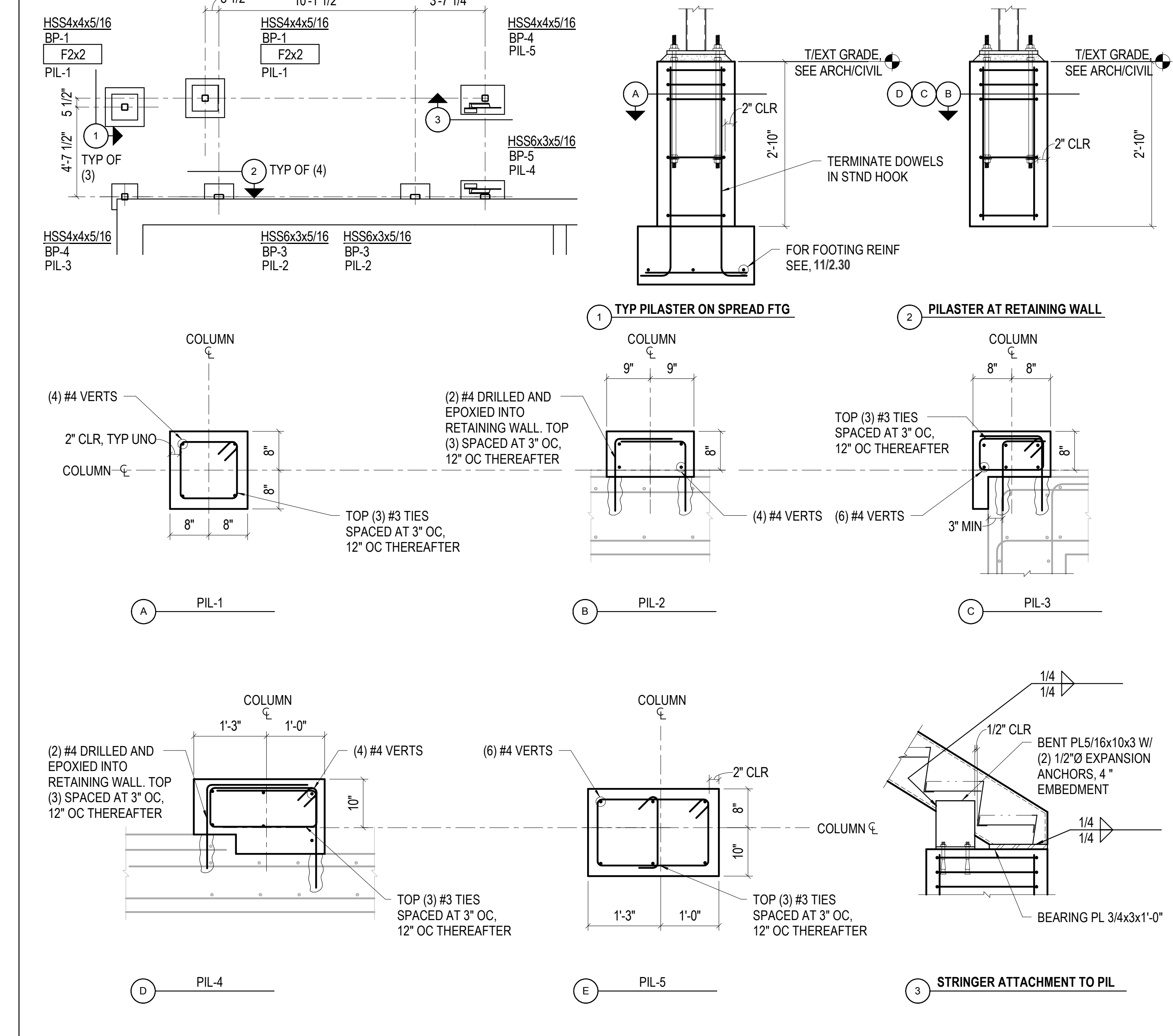
20 NO SCALE FOUNDATION DETAILS AT STAIRS
