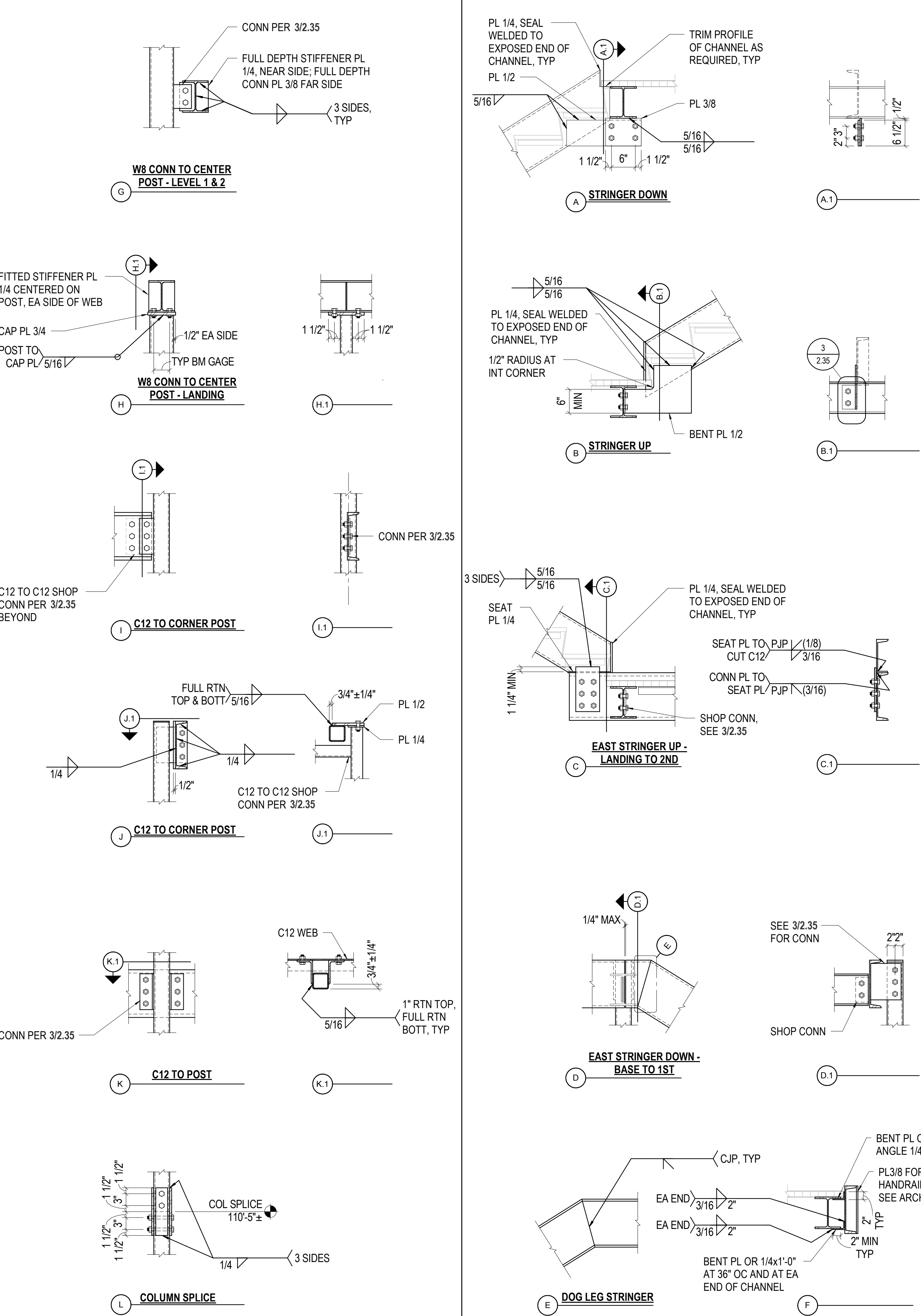
12 NO SCALE STAIR LANDINGS TO COLUMN & COLUMN DETAILS
