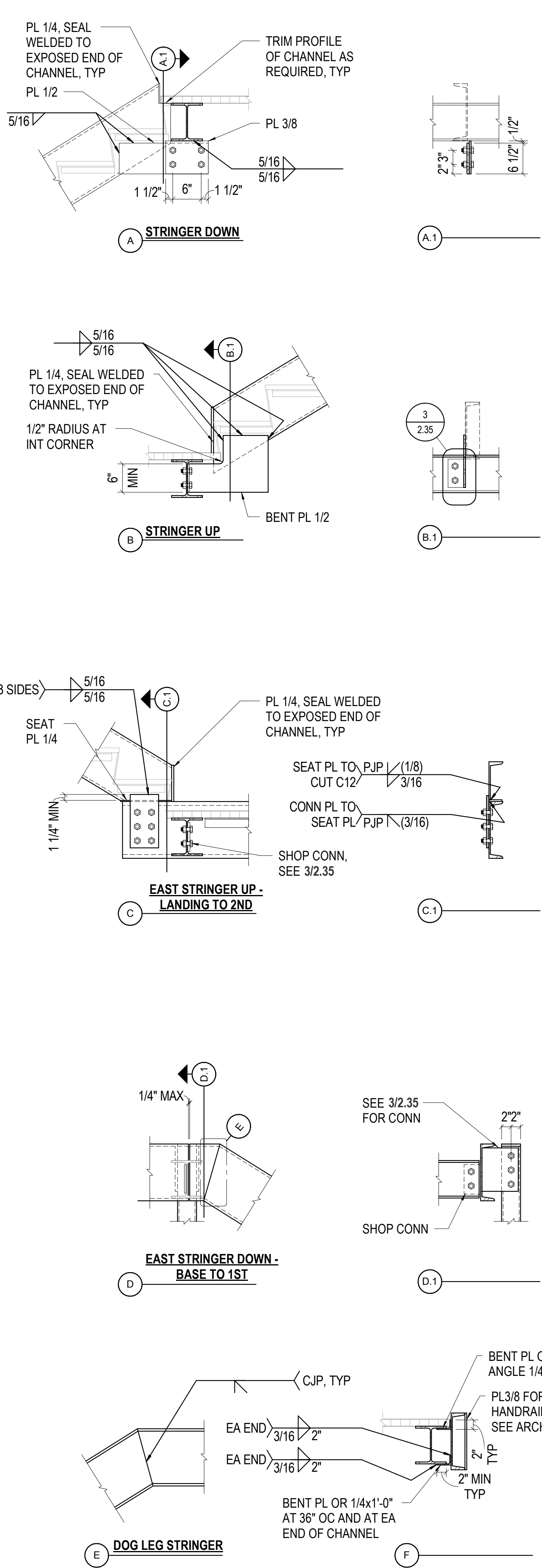
8 NO SCALE STAIR STRINGERS TO LANDINGS
