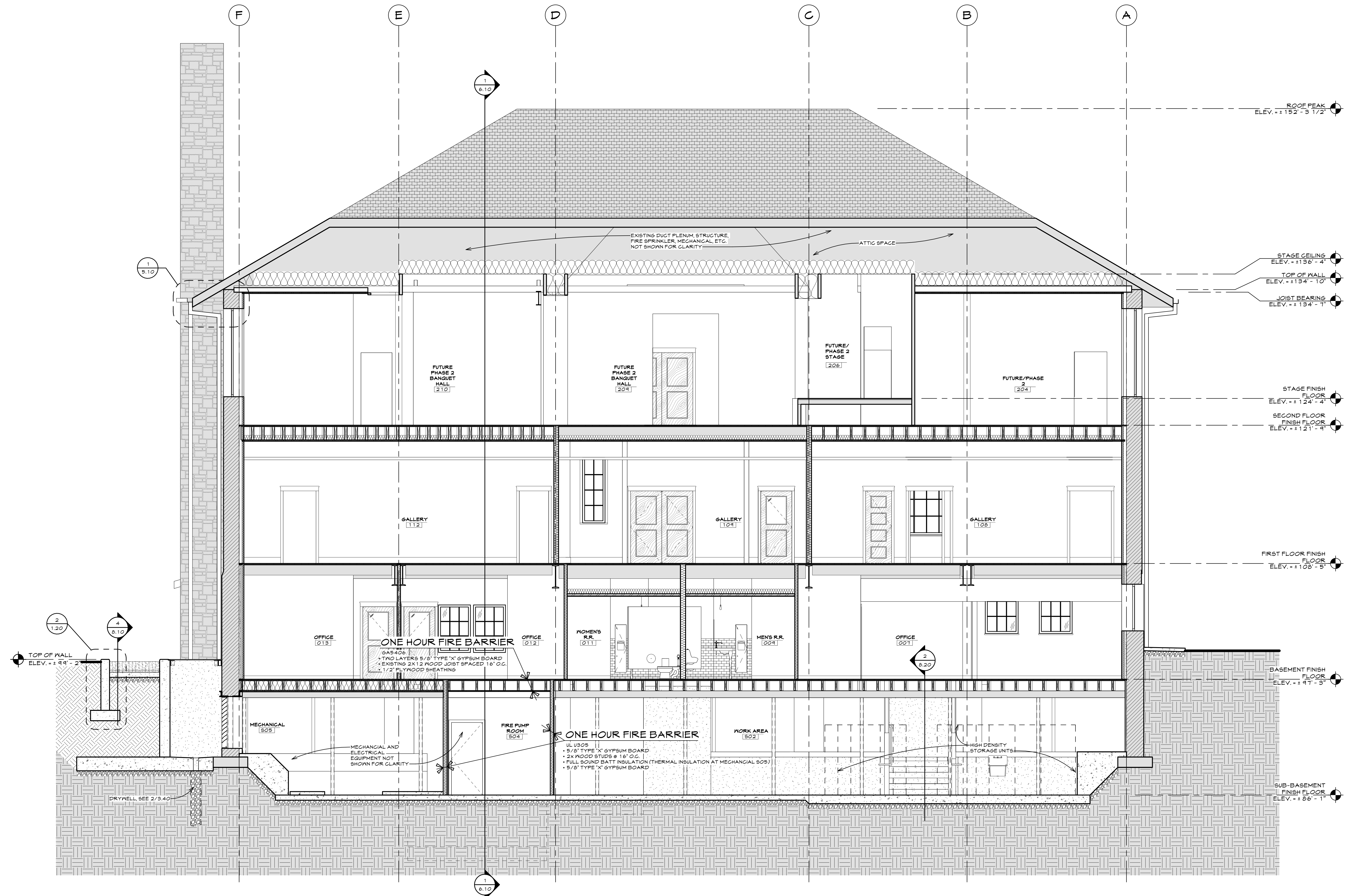
1 BUILDING SECTION 2 SCALE: 1/4" = 1'-0"
