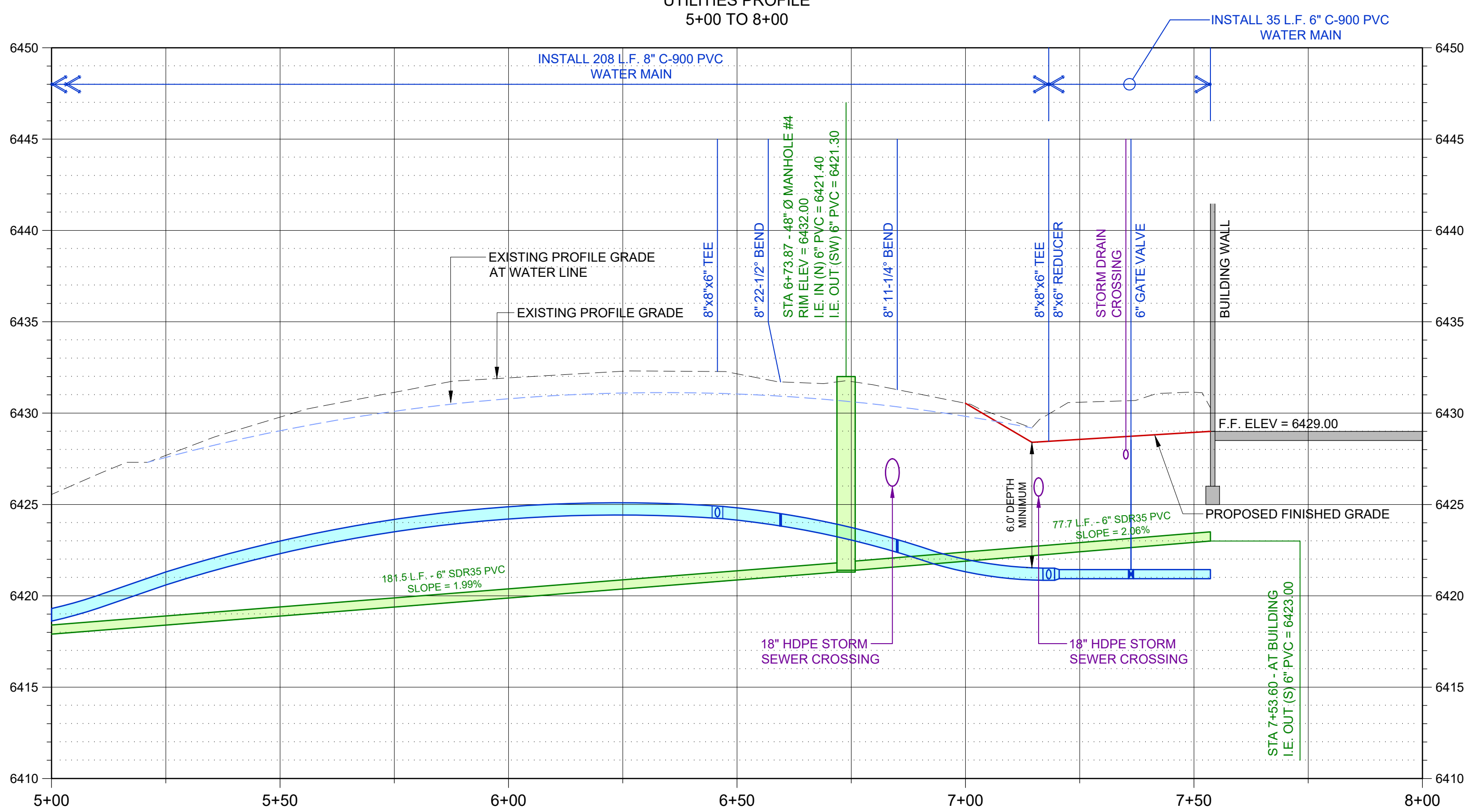
WATER AND SANITARY SEWER SERVICES
