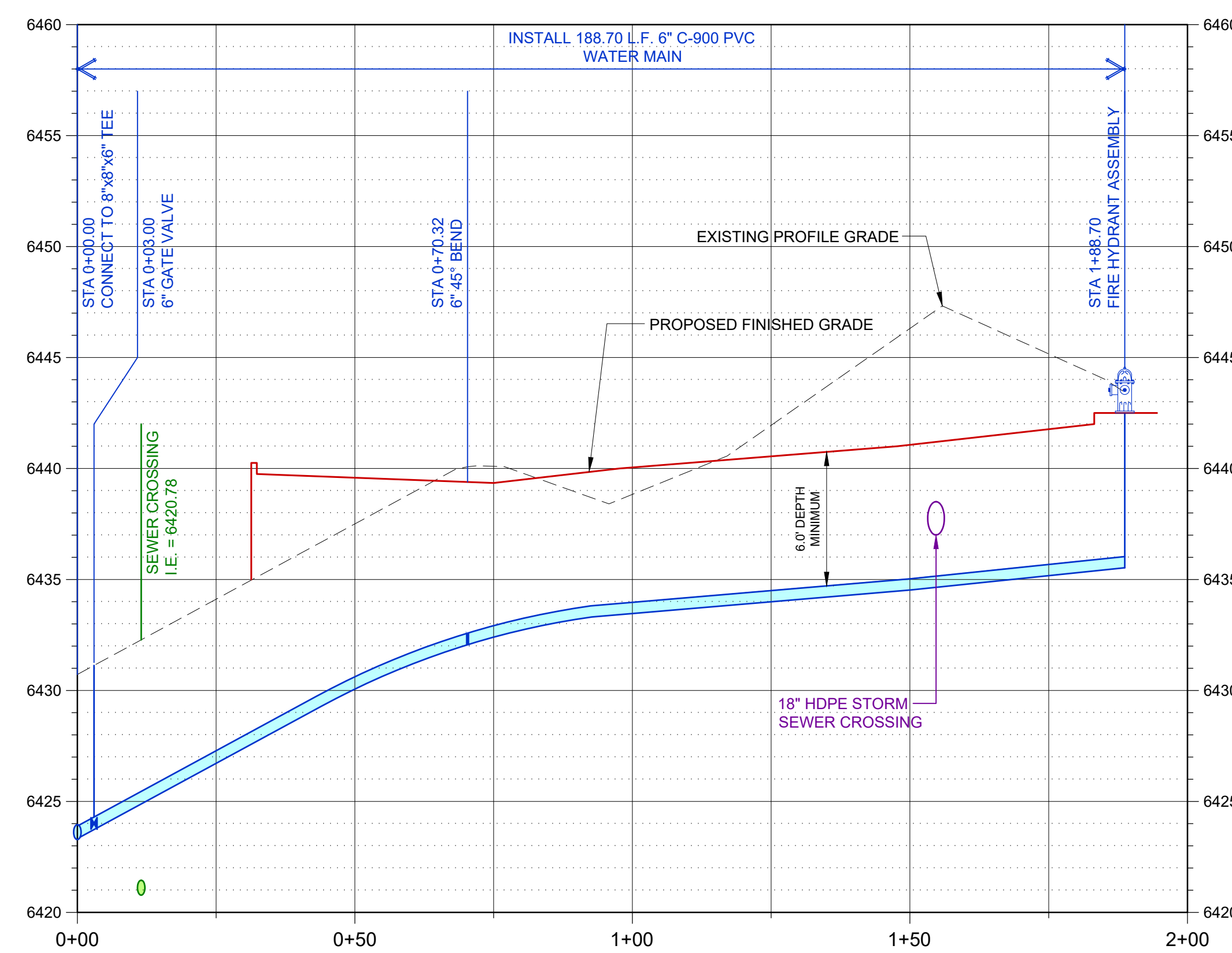
FIRE HYDRANT LEAD #1
