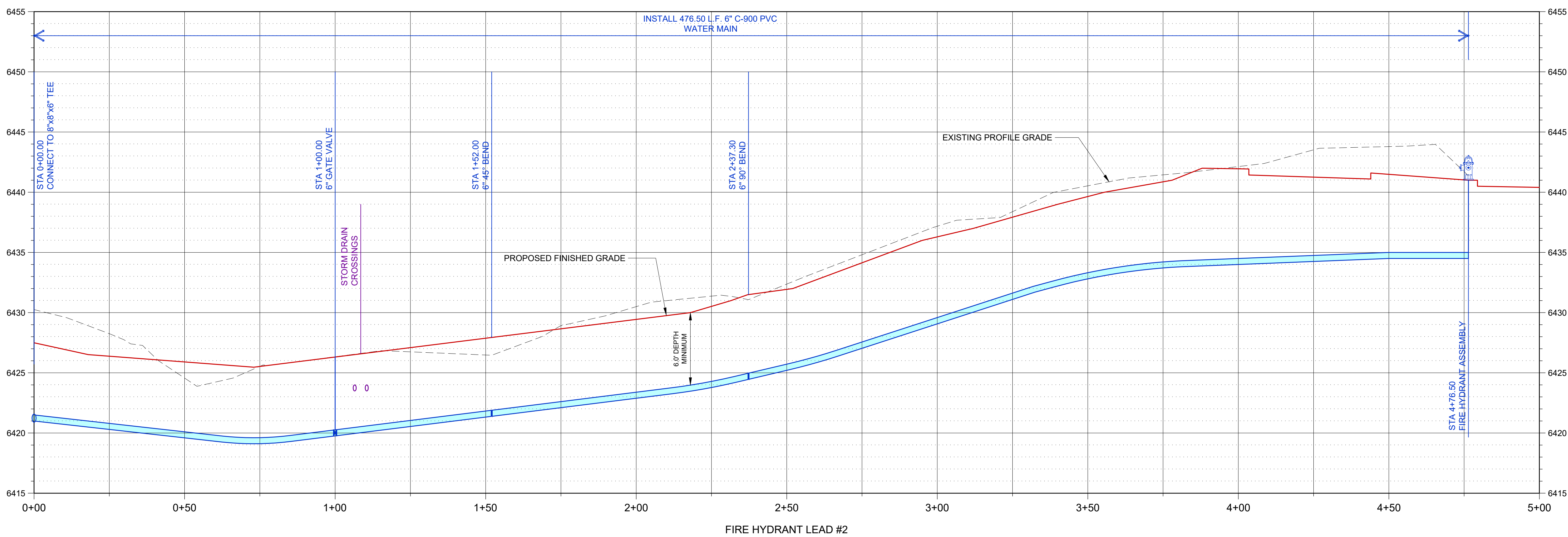
UTILITIES PROFILE 0+00 TO 5+00
