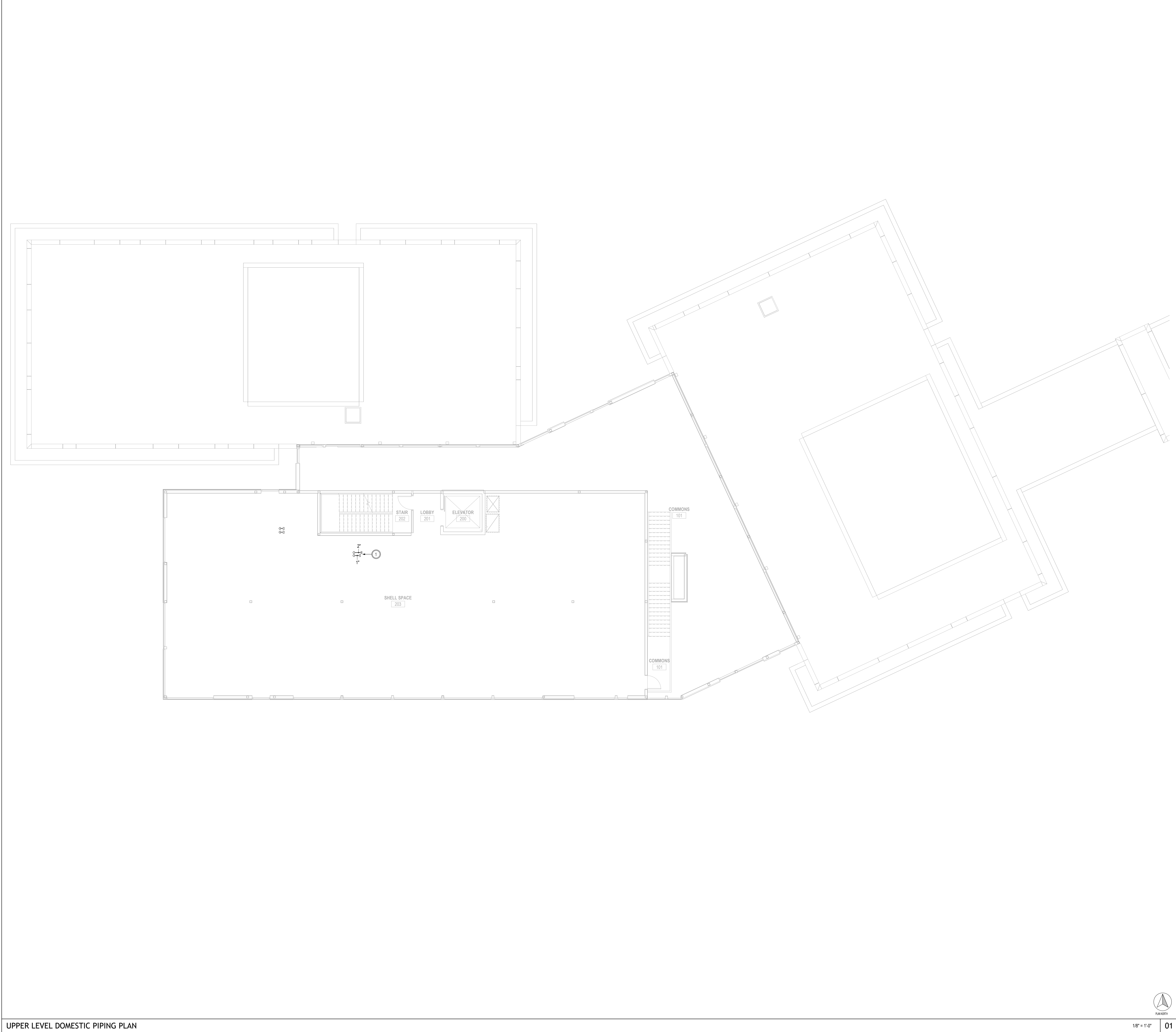
UPPER LEVEL DOMESTIC PIPING PLAN
