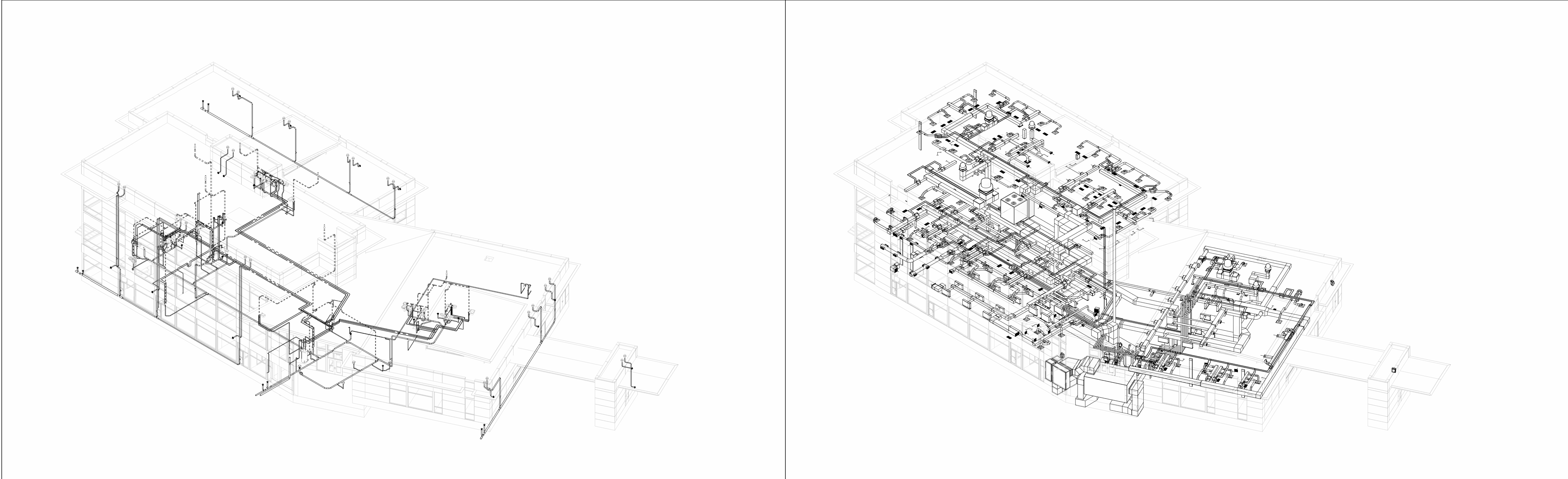
PLUMBING SCHEMATIC RISER DIAGRAM NO SCALE 39 HVAC SCHEMATIC RISER DIAGRAM NO SCALE 38
