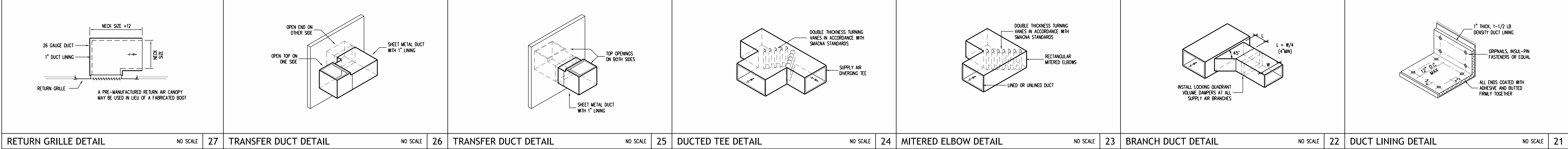
RETURN GRILLE DETAIL NO SCALE 27 TRANSFER DUCT DETAIL NO SCALE 26 TRANSFER DUCT DETAIL NO SCALE 25 DUCTED TEE DETAIL NO SCALE 24 MITERED ELBOW DETAIL NO SCALE 23 BRANCH DUCT DETAIL NO SCALE 22 DUCT LINING DETAIL NO SCALE 21
