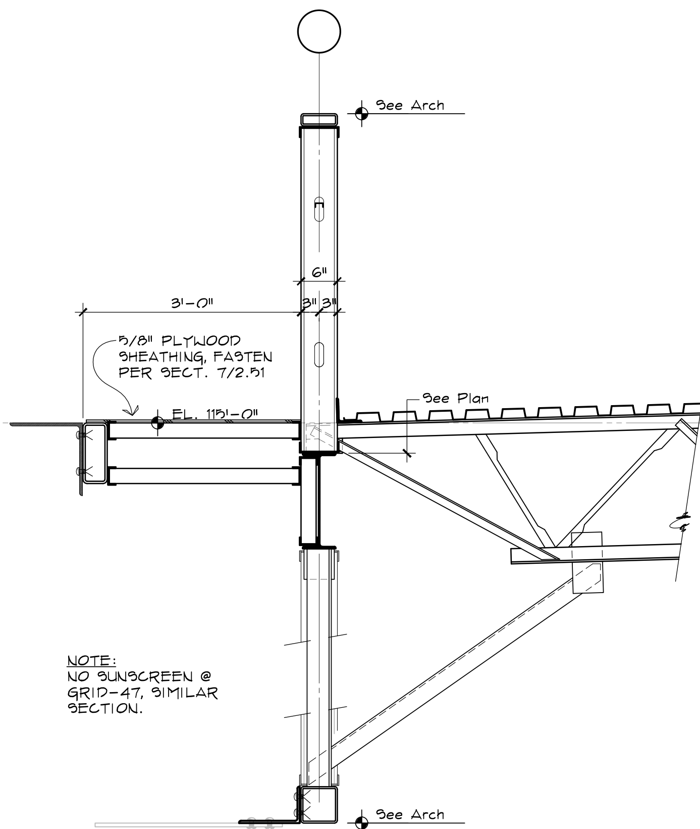
2 SECTION 2.12 3/4" = 1'-0"
