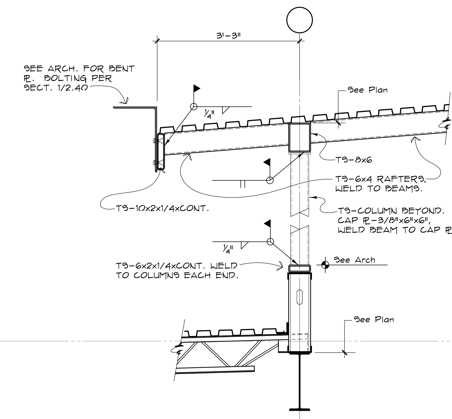
8 SECTION 2.12 3/4" = 1'-0"
