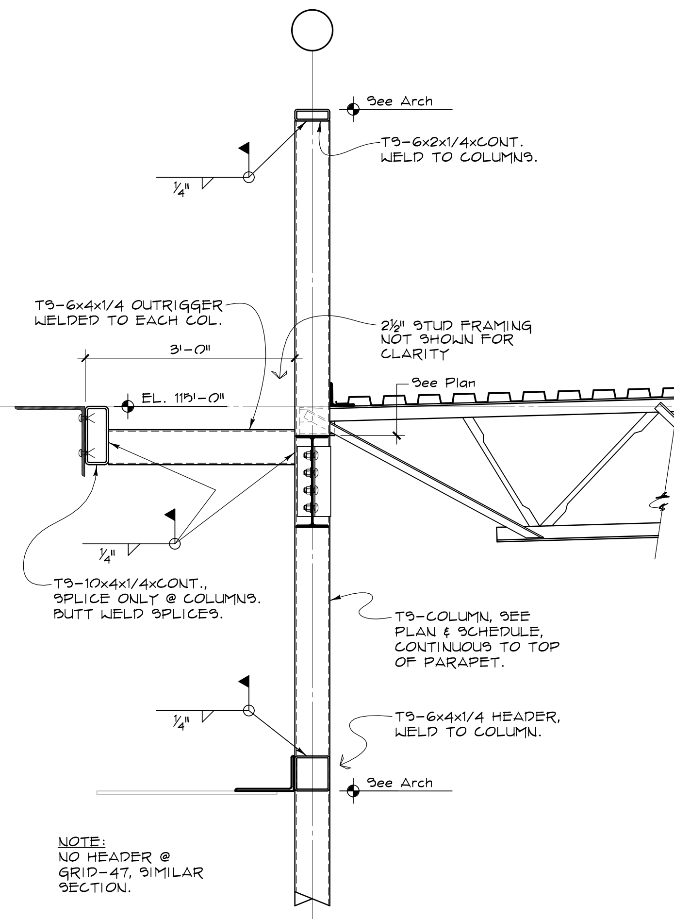
3 SECTION 2.12 3/4" = 1'-0"
