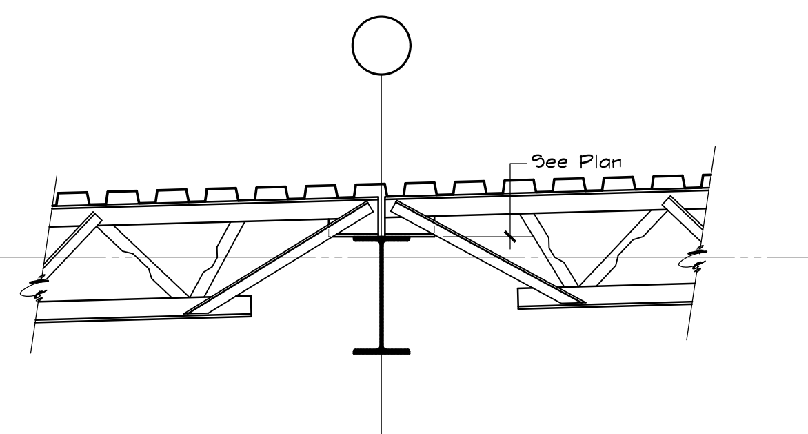
6 SECTION 2.12 3/4" = 1'-0"
