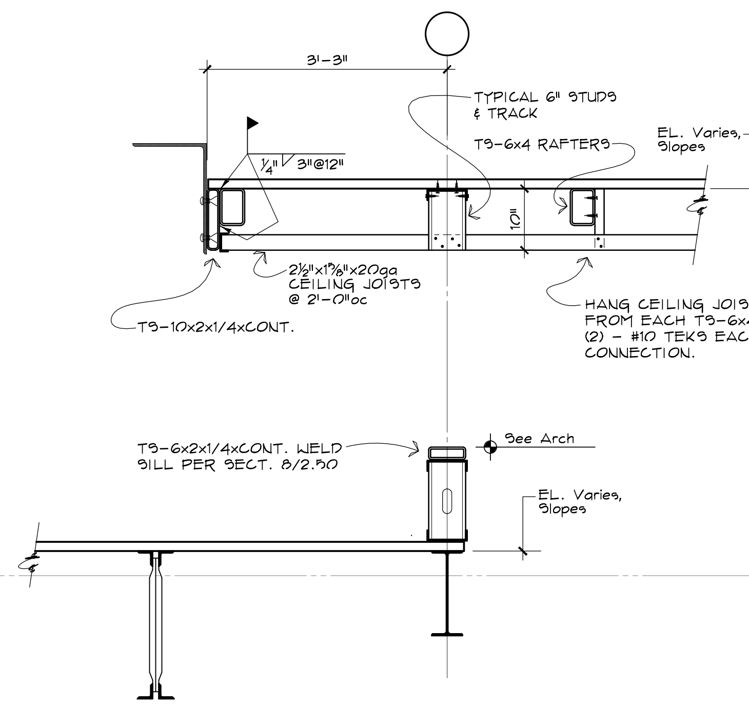
7 SECTION 2.12 3/4" = 1'-0"
