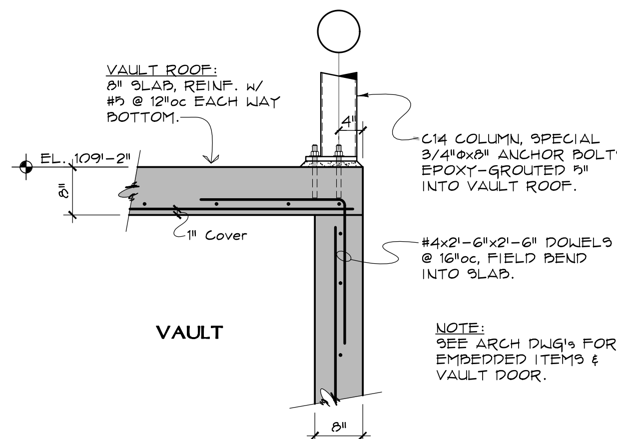
9 SECTION 2.12 3/4" = 1'-0"
