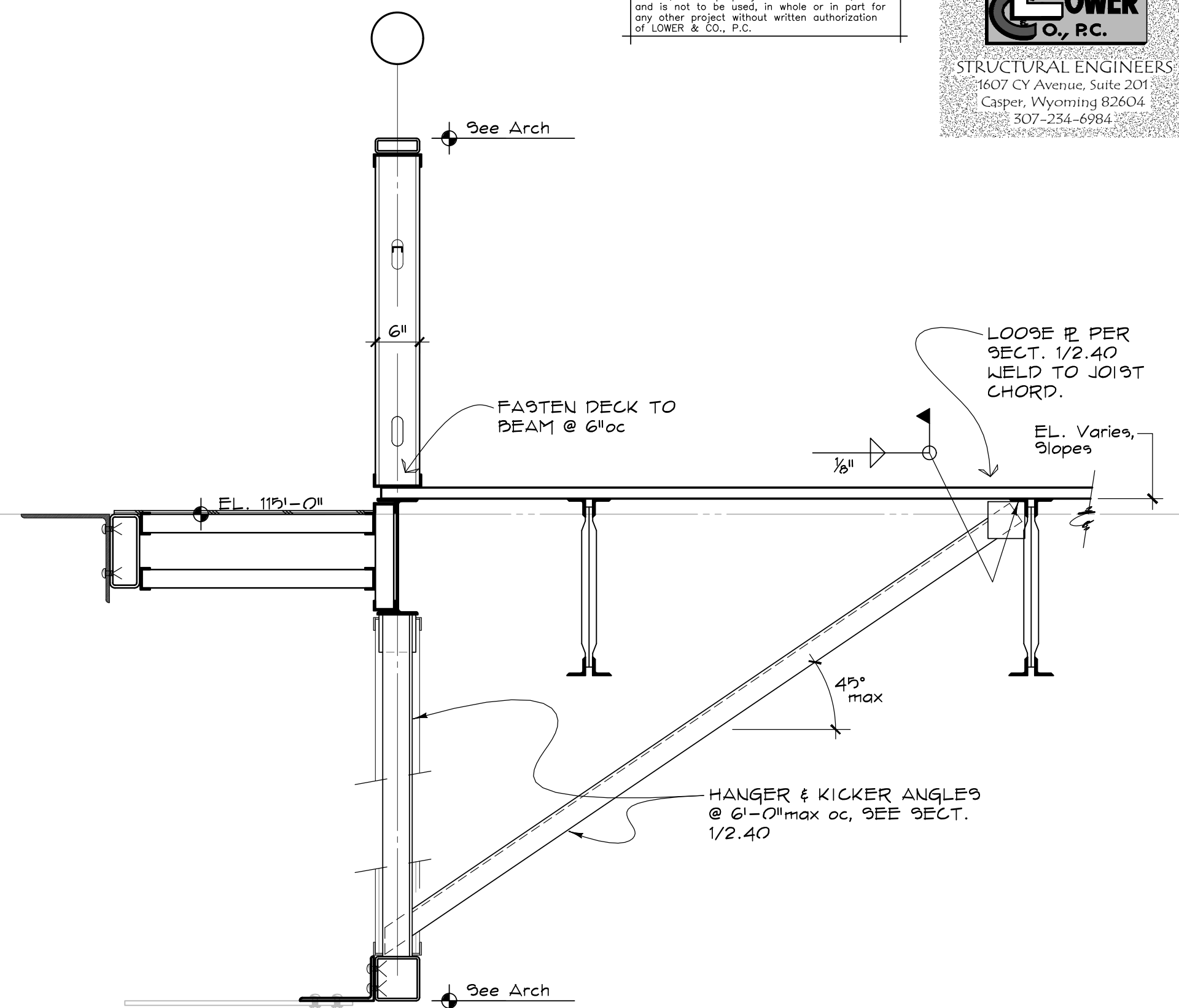
4 SECTION 2.12 3/4" = 1'-0"
