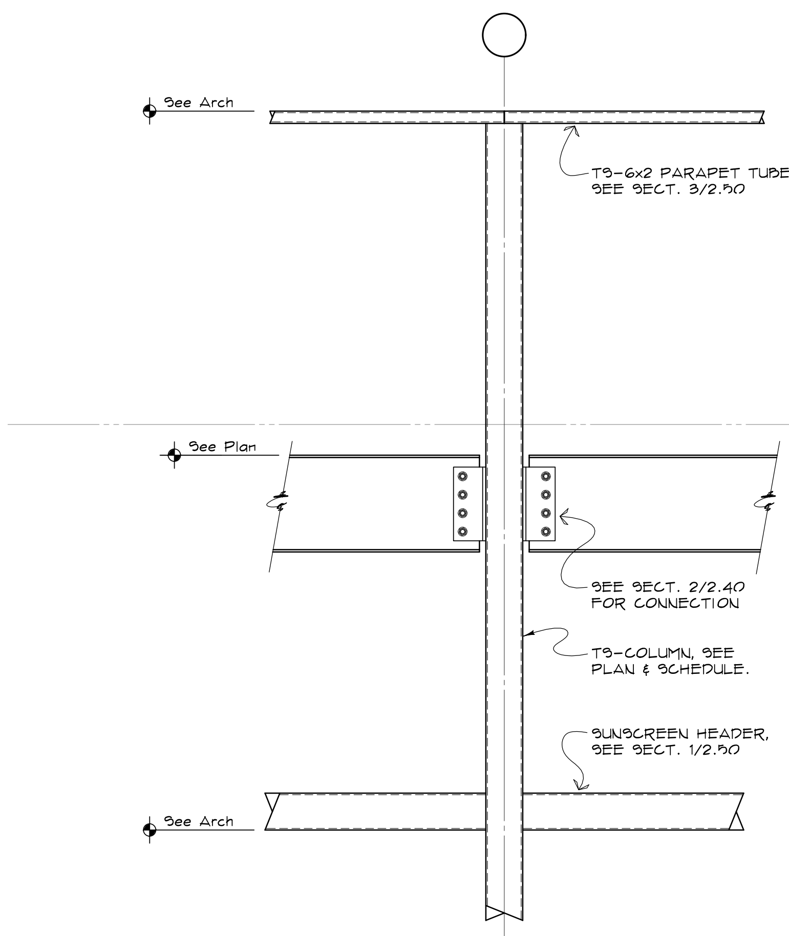
5 SECTION 2.12 3/4" = 1'-0"
