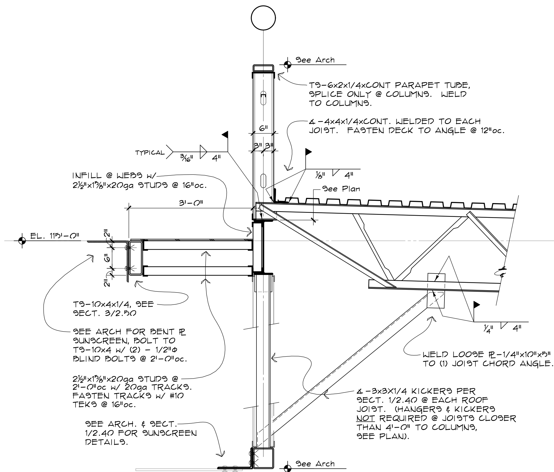
1 SECTION 2.12 3/4" = 1'-0"
