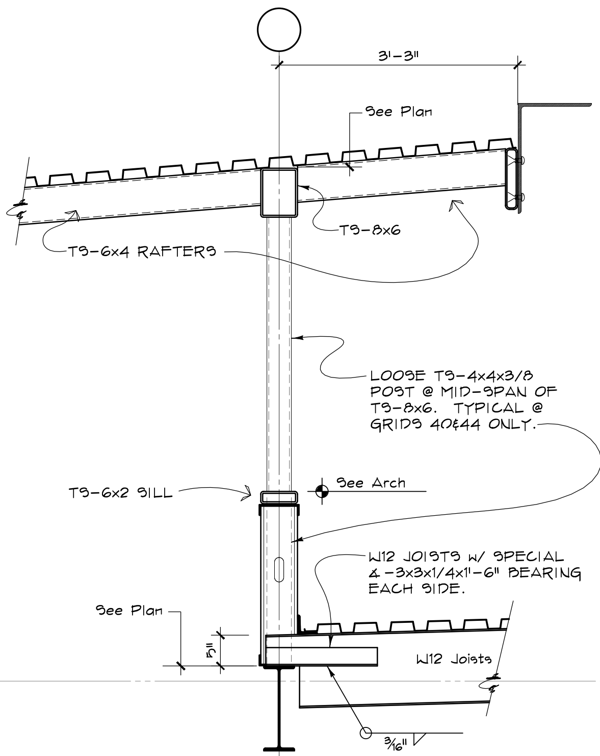
2 SECTION 2.12 3/4" = 1'-0"
