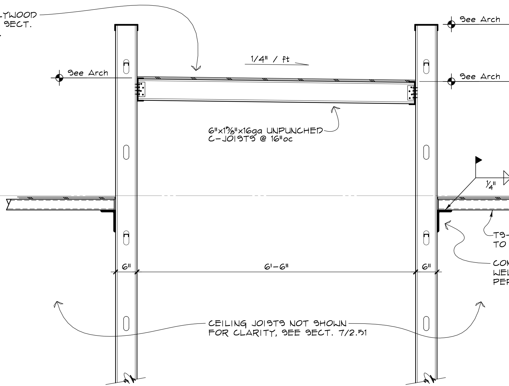
6 SECTION 2.12 3/4" = 1'-0"
