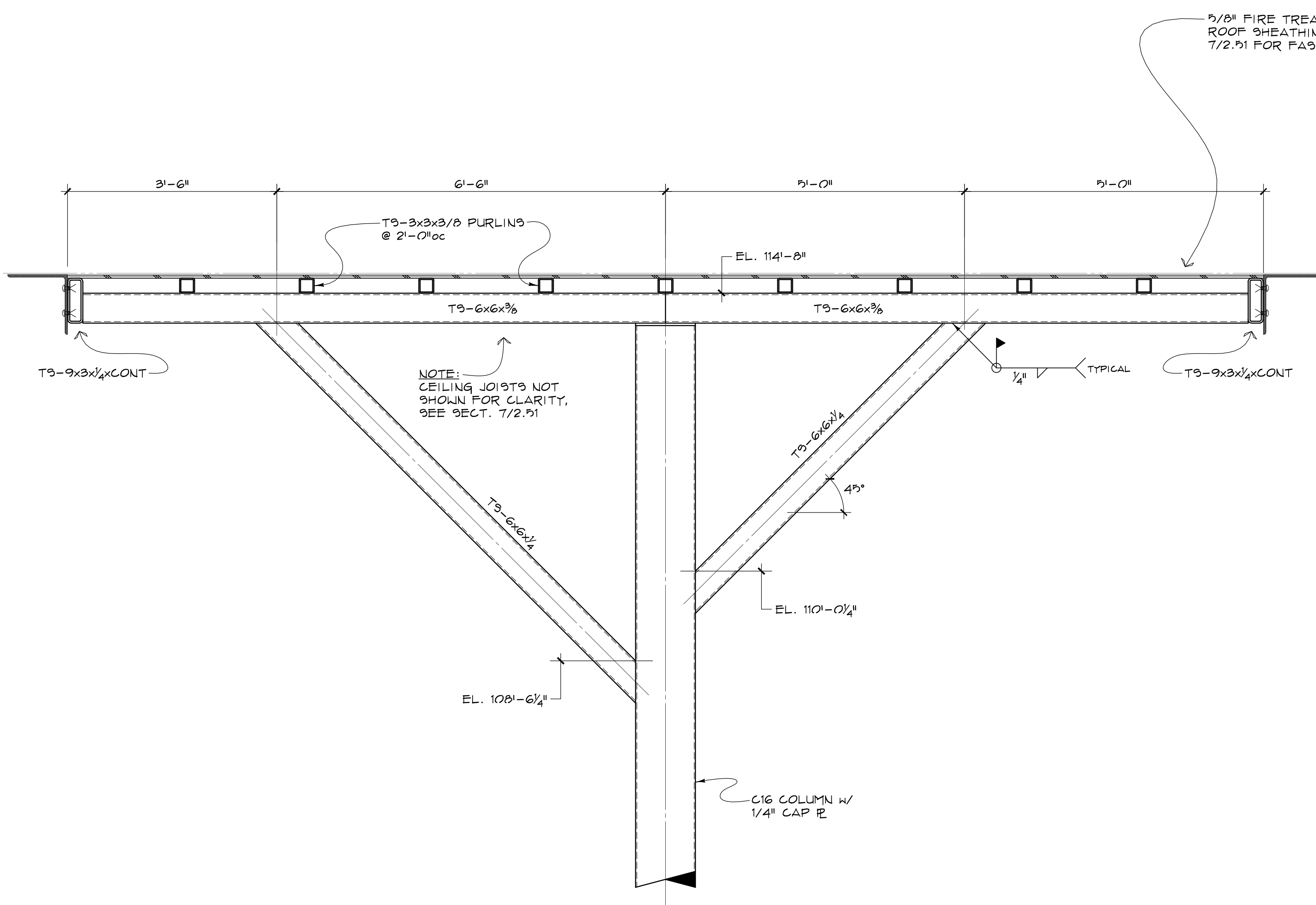
5 SECTION 2.12 3/4" = 1'-0"
