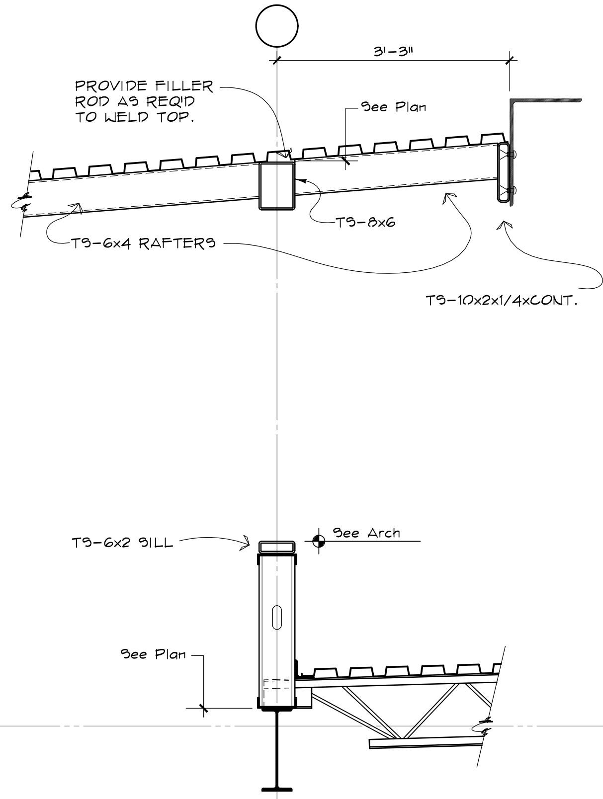
1 SECTION 2.12 3/4" = 1'-0"
