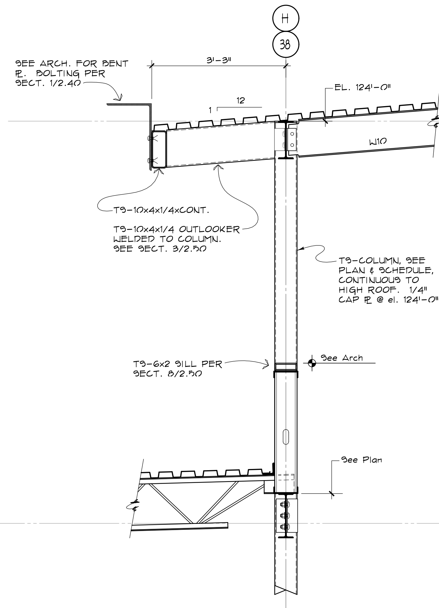
3 SECTION 2.12 3/4" = 1'-0"
