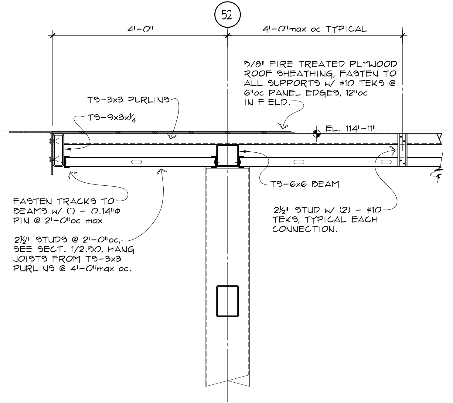
7 SECTION 2.12 3/4" = 1'-0"
