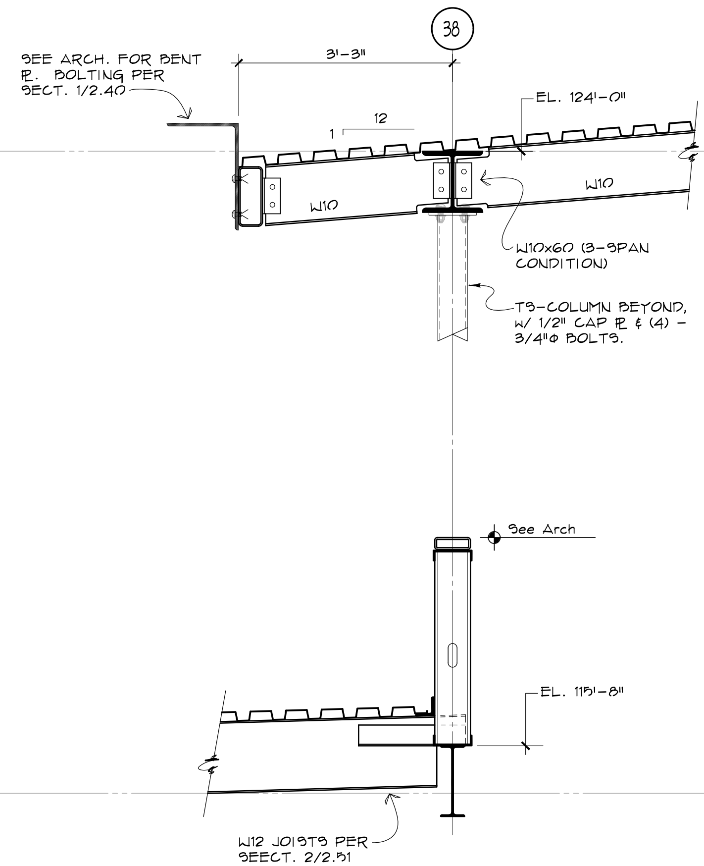
4 SECTION 2.12 3/4" = 1'-0"
