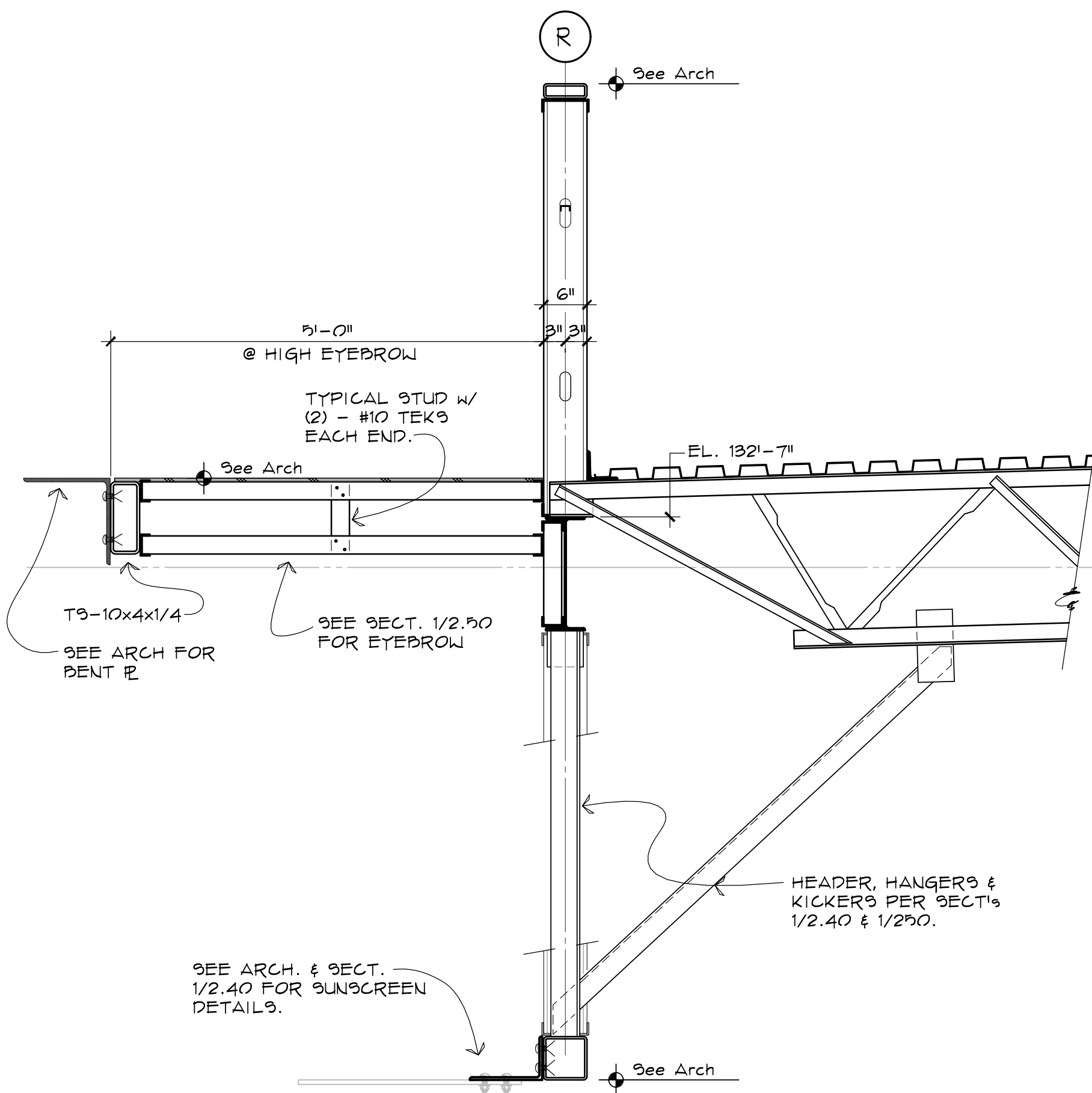
SECTION 1 2.13 3/4" = 1'-0"
