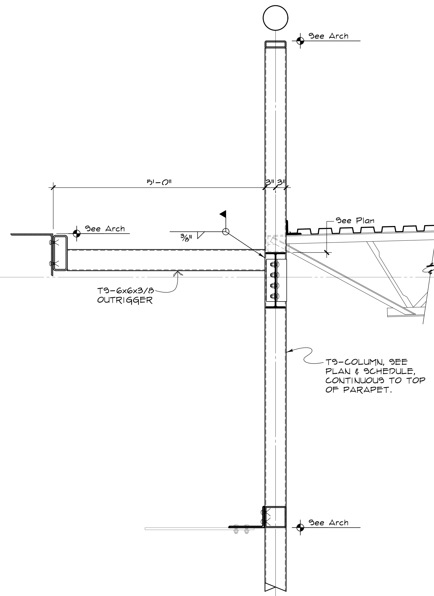
SECTION 3 2.13 3/4" = 1'-0"
