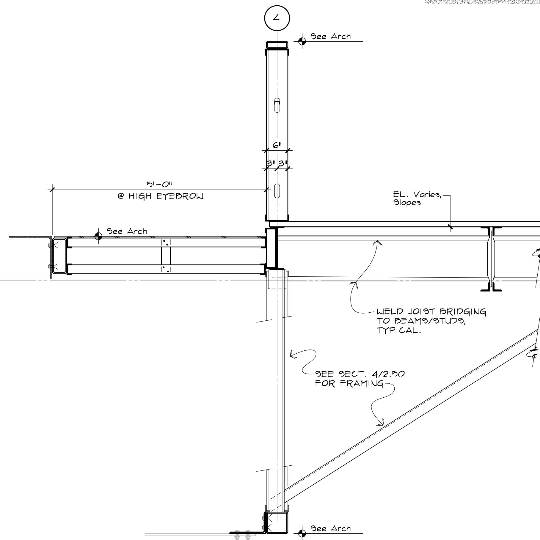
SECTION 4 2.13 3/4" = 1'-0"
