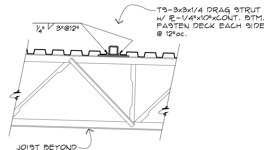
SECTION 9 2.13 3/4" = 1'-0"
