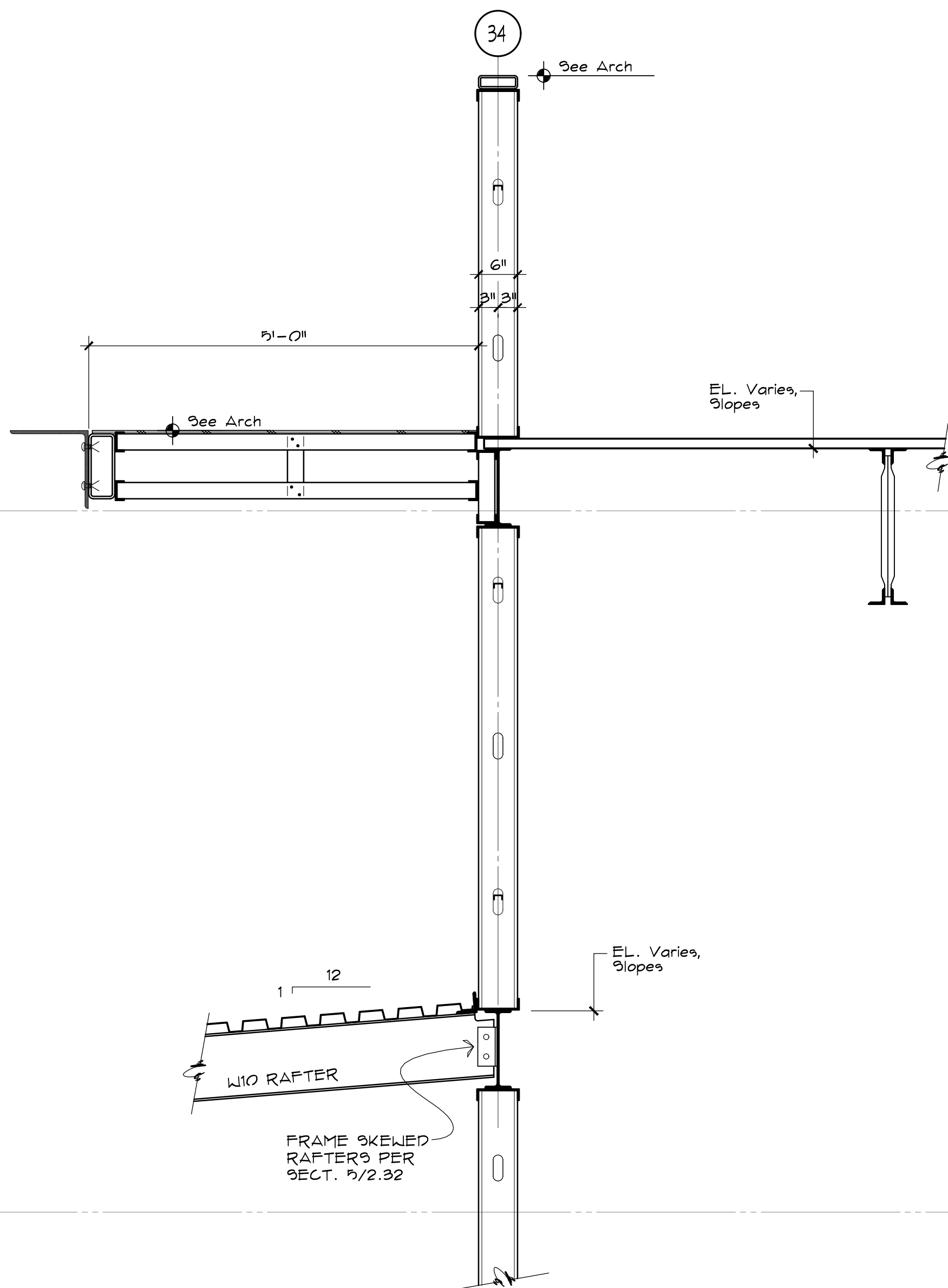
SECTION 6 2.13 3/4" = 1'-0"
