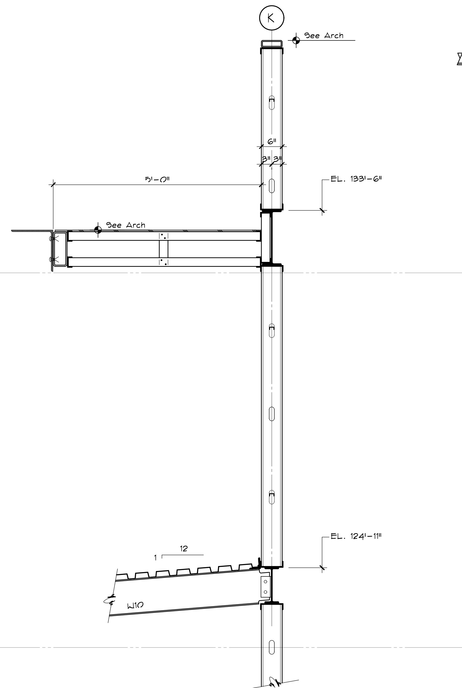
SECTION 7 2.13 3/4" = 1'-0"
