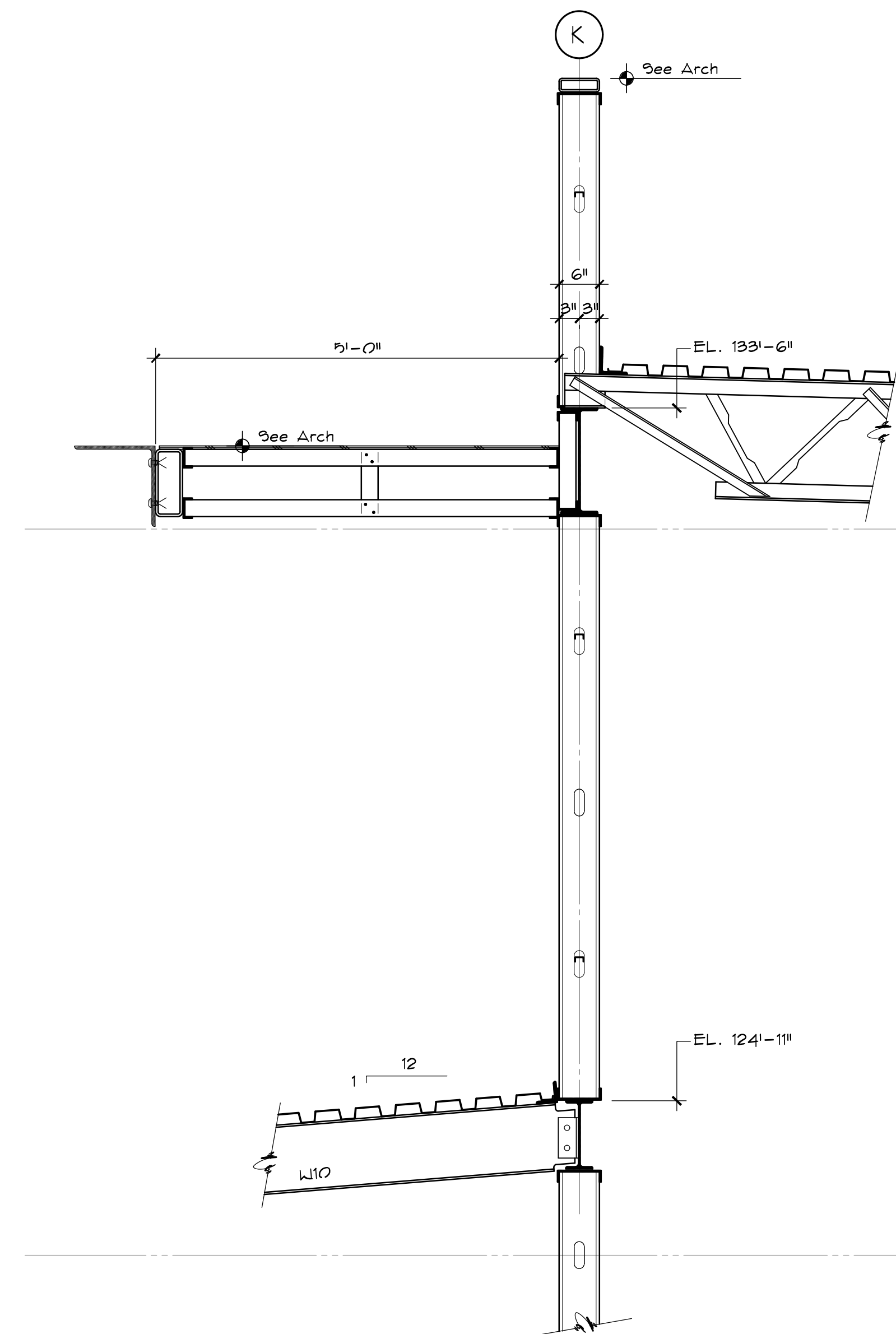
SECTION 5 2.13 3/4" = 1'-0"
