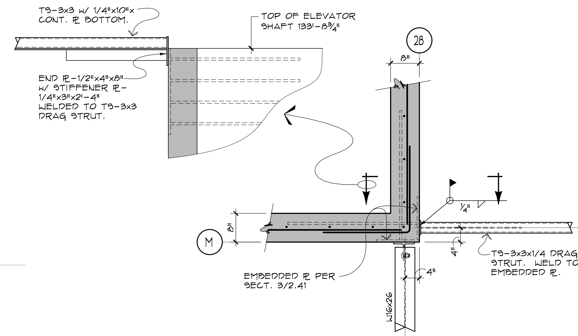
DETAIL 8 2.13 3/4" = 1'-0"
