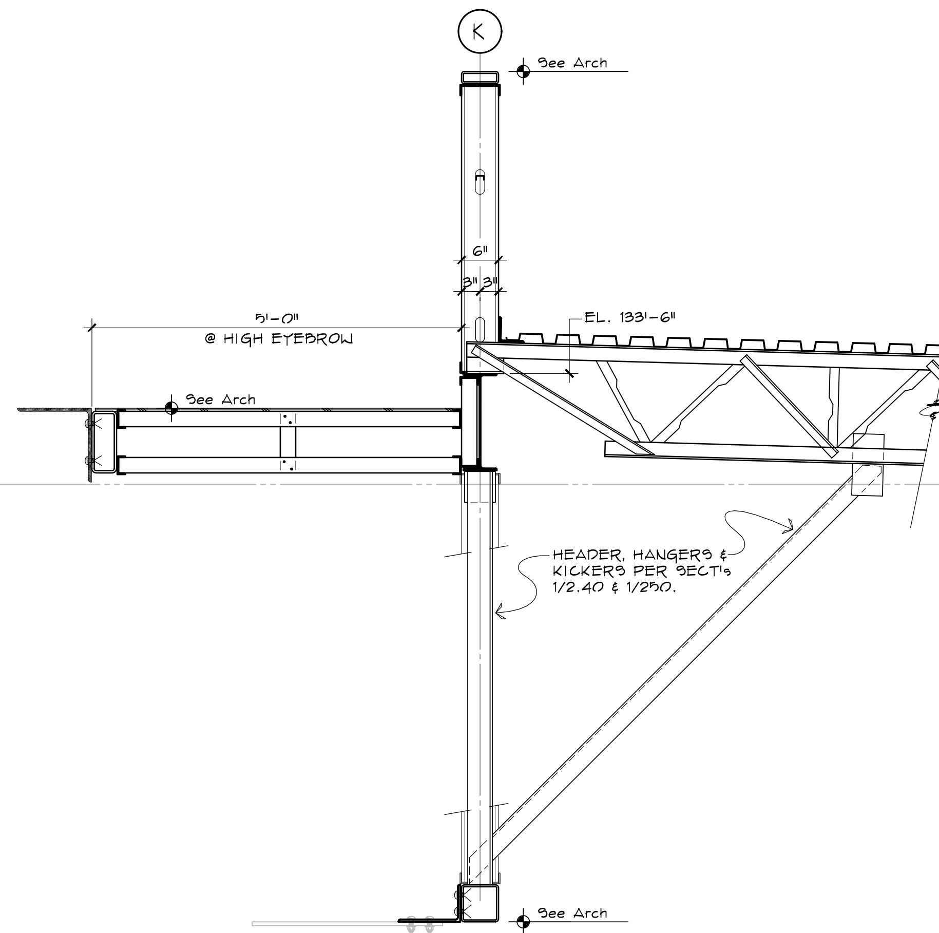
SECTION 2 2.13 3/4" = 1'-0"
