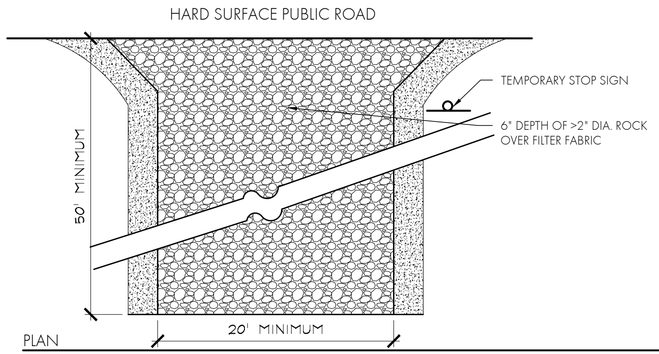
1 VEHICLE TRACKING CONTROL
