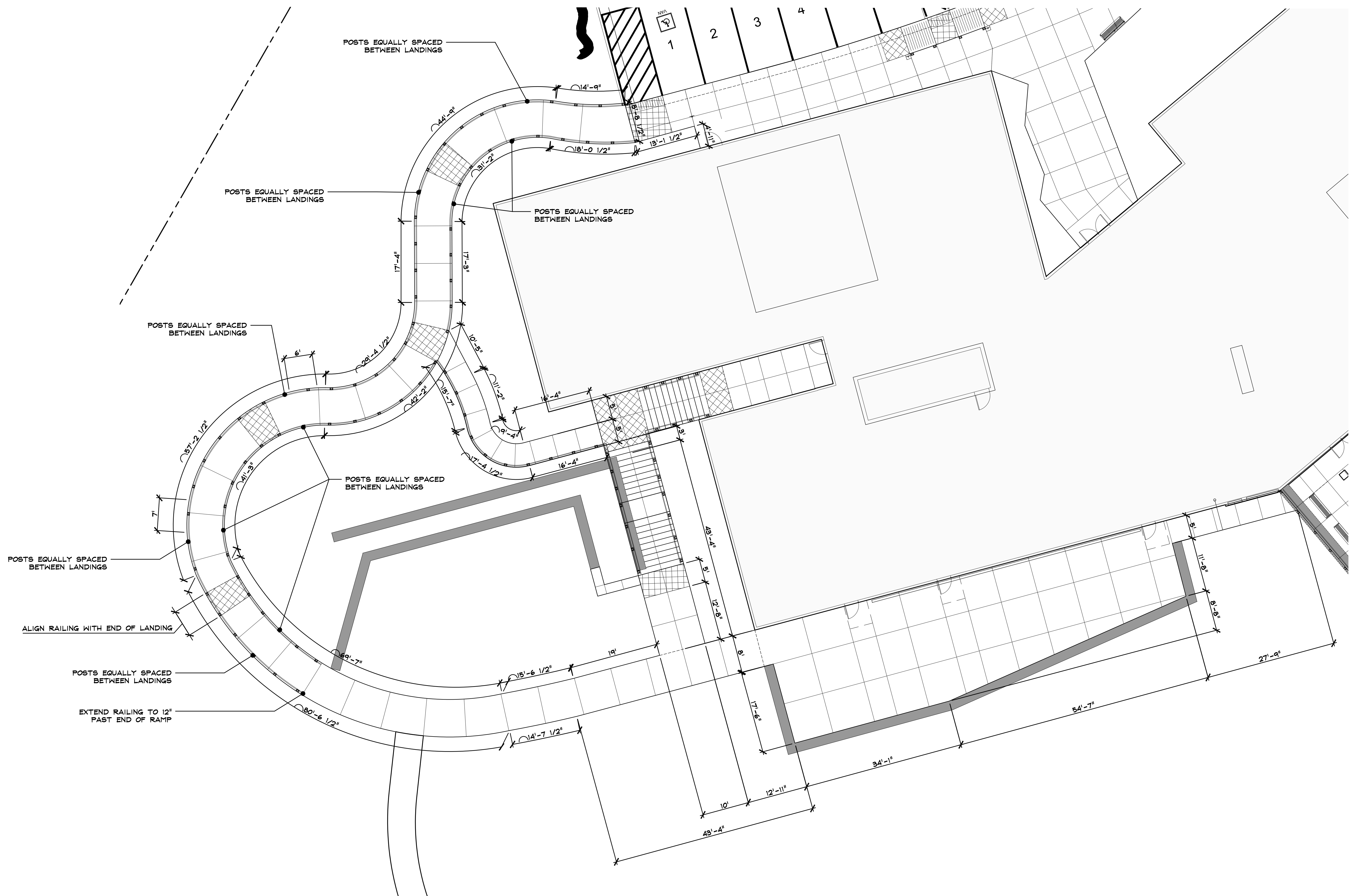
DETAILED LAYOUT PLAN: LOWER PATIO AND LAWN
